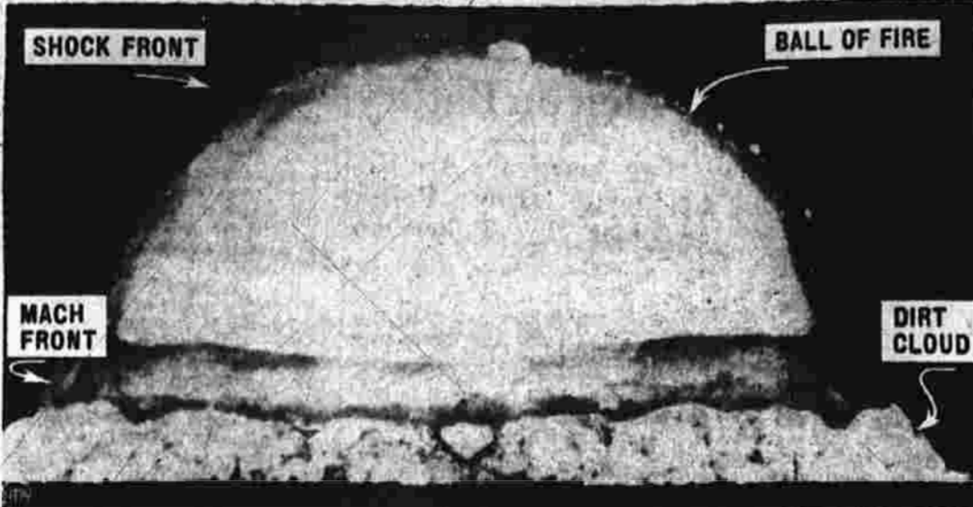
Blinding light, hot as the sun: Illustration from the AEC's new atomic weapons handbook shows ball of fire touching ground soon after "breakaway" in "Trinity" A-bomb test at Alamogordo, N. M. Shock front, "Mach front" due to shock wave refraction, and dirt cloud are indicated.
